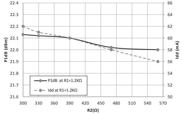
Figure 19. P1dB and Quiescent Current with different R2 [1]
