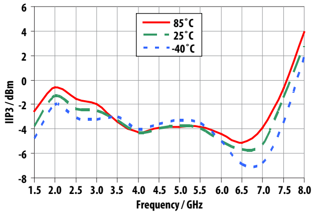
Figure 21. IIP3 vs Frequency
