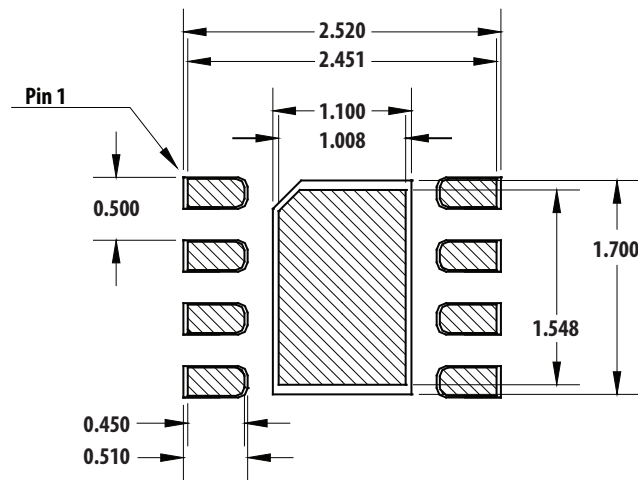
Combined Land Pattern and Stencil Layout
