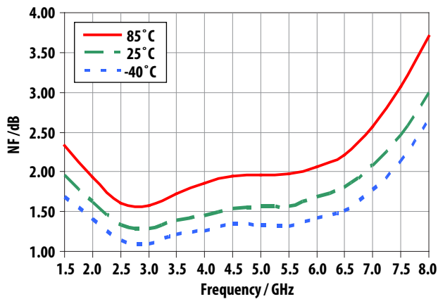
Figure 37. Noise Figure vs Frequency
