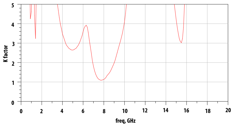
Figure 49. K factor vs Frequency
