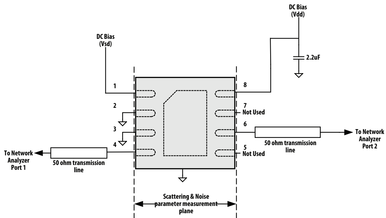
Figure 50. Scattering and Noise parameter test circuit
