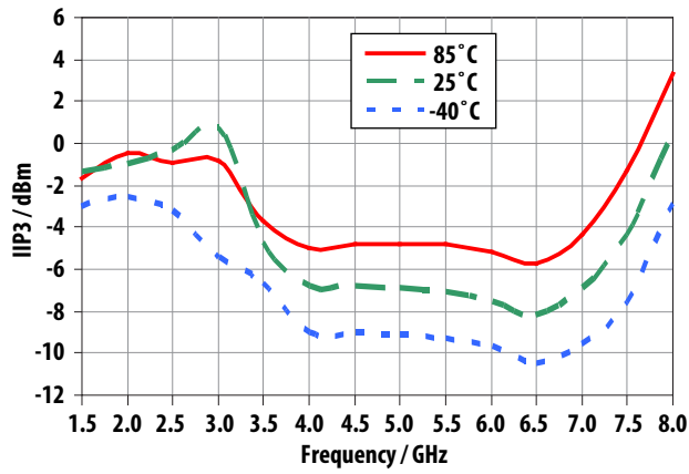
Figure 15. IIP3 vs Frequency
