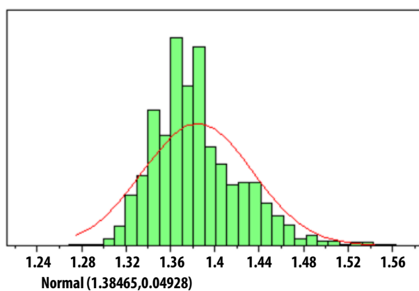
Figure 2. NF (dB) at 3.5 GHz, Vdd 1.4V; Vsd 1.4 V
