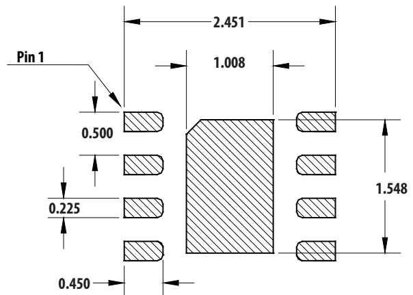
Stencil Opening
