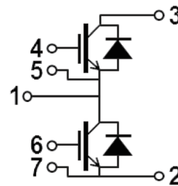
Circuit Diagram and Pin Assignment
