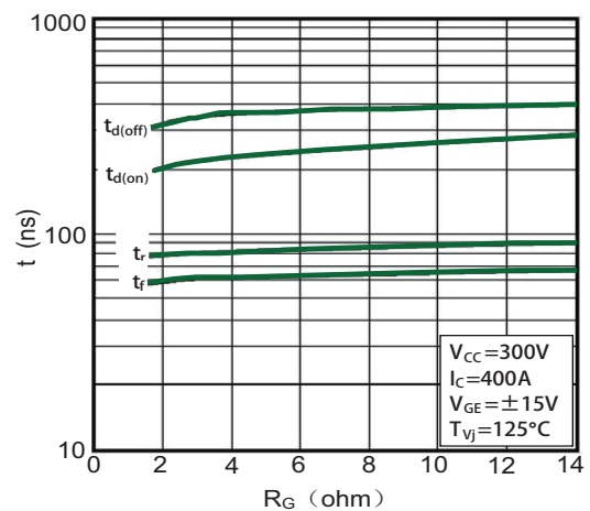
Figure 6: Switching Times vs. Gate Resistor
