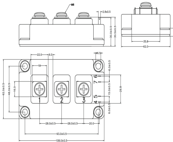
Dimensions-Package D
