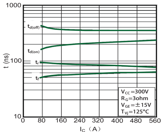
Figure 5: Switching Times vs. Collector Current
