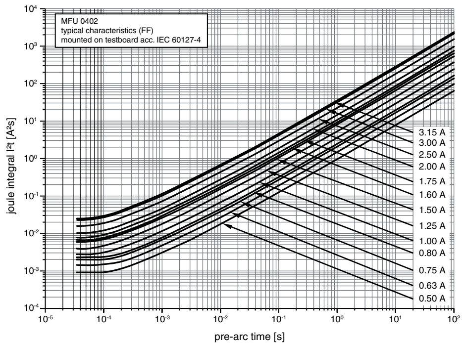
Typical I^2t vs. t Characteristic of MFU 0402
