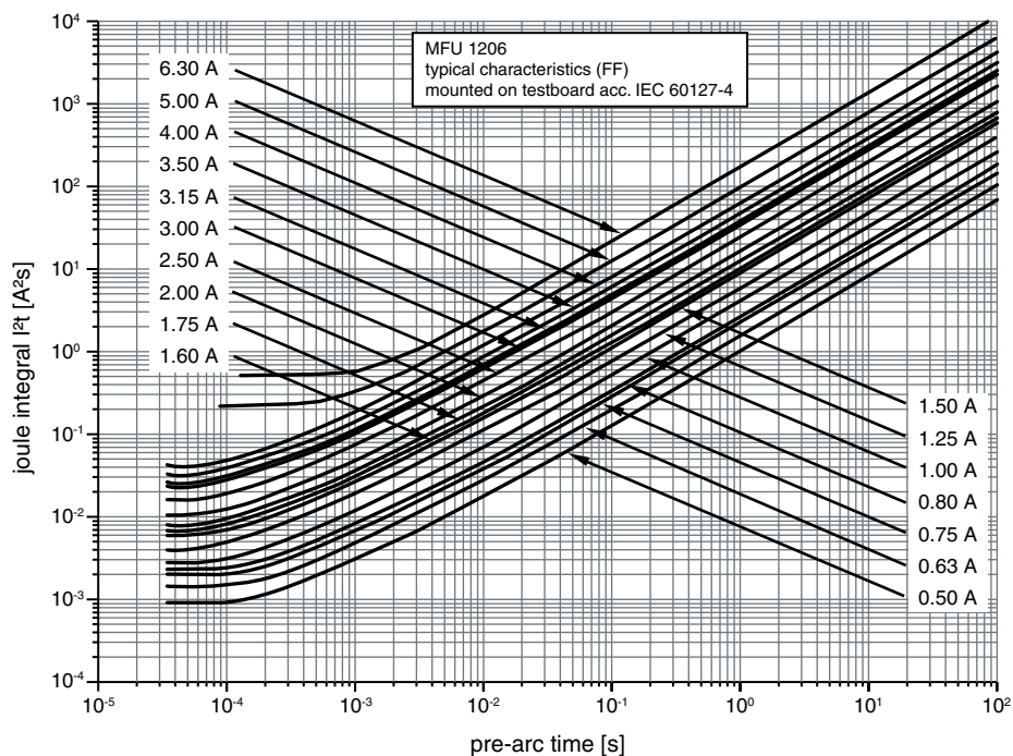
Typical I^2t vs. t Characteristic of MFU 1206
