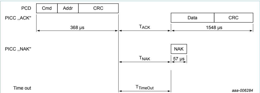
Figure 13. READ command
