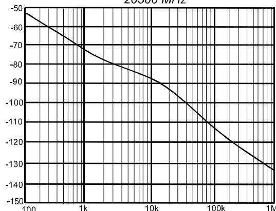
Phase Noise (dBc/Hz) 20500 MHz
