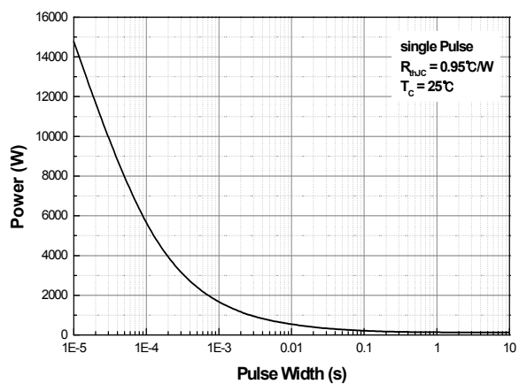
Fig.13 Single Pulse Maximum Power Dissipation MDP6N60(TO-220)
