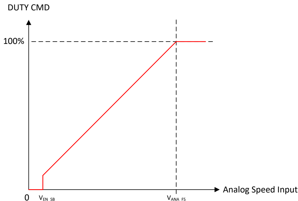
Figure 8-16. Analog-Mode Speed Control
