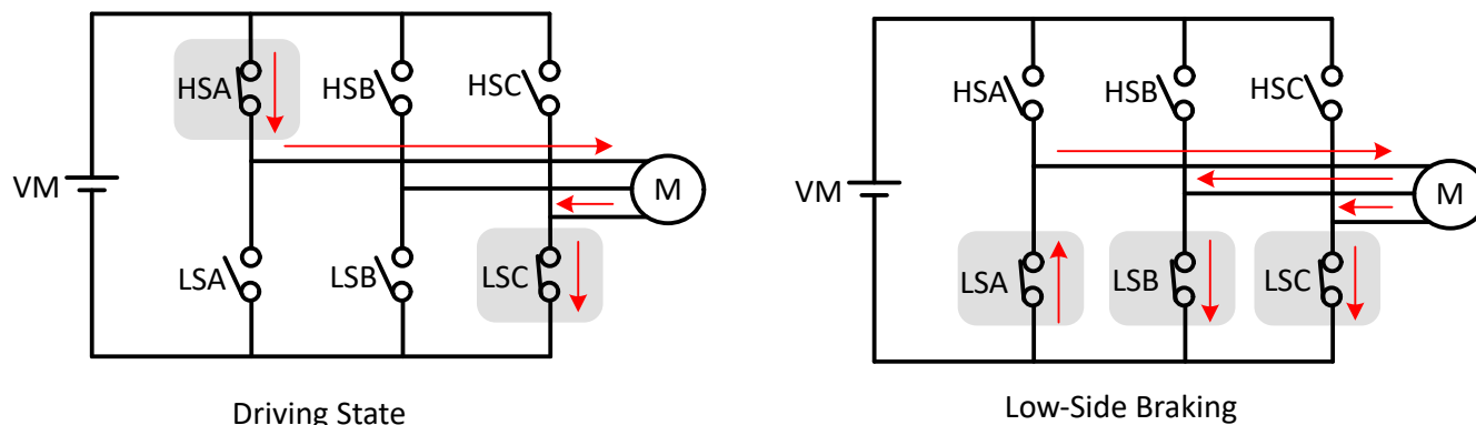
Figure 8-43. Low-Side Braking
