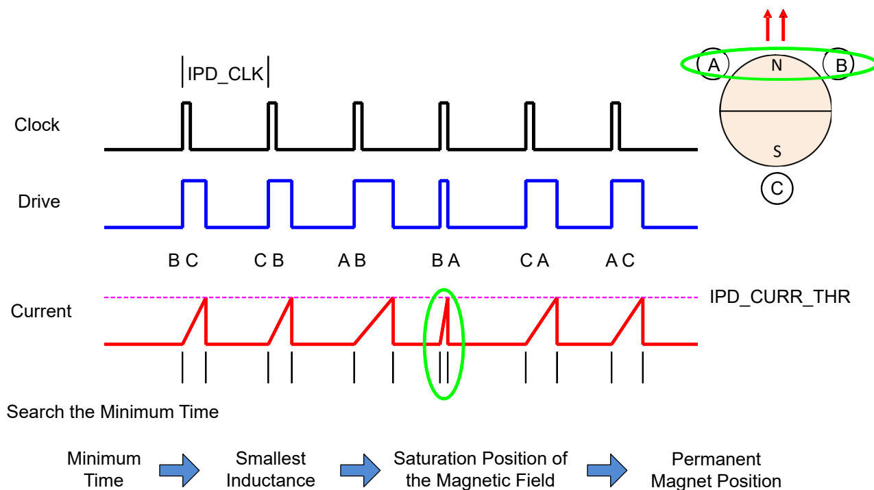
Figure 8-21. IPD Function
