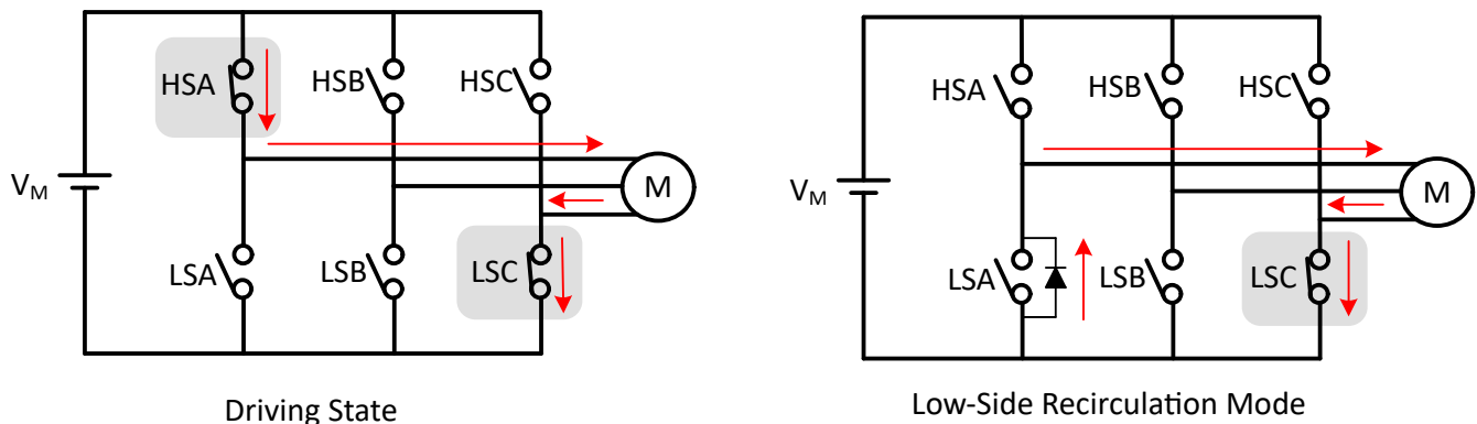
Figure 8-41. Low-Side Recirculation
