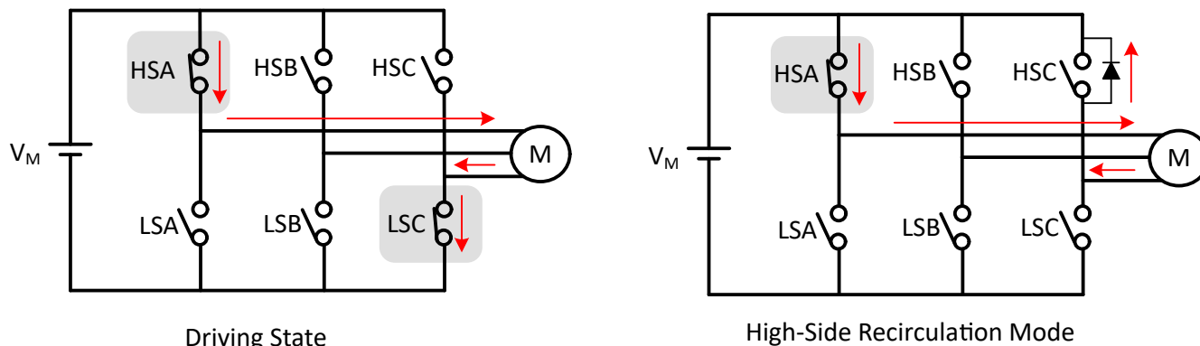
Figure 8-42. High-Side Recirculation
