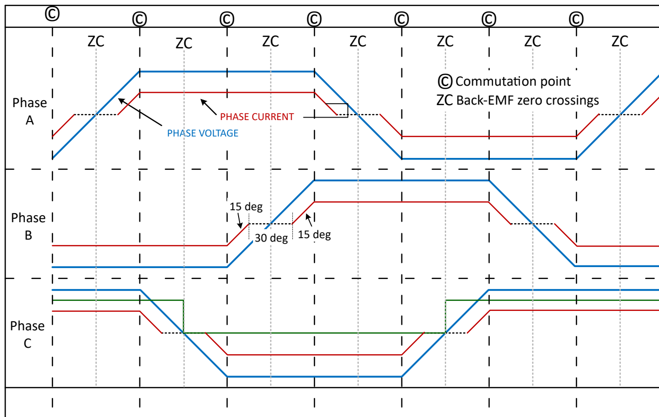
Figure 8-29. 150° commutation
