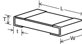
Wraparound Termination (standard)
