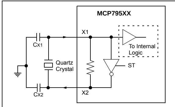
FIGURE 5-3: CRYSTAL OPERATION
