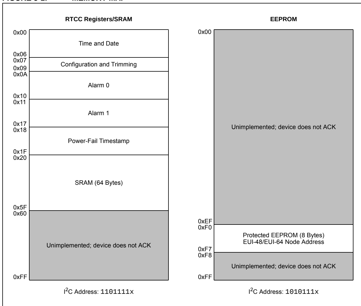
FIGURE 5-1: MEMORY MAP
