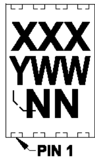
8-Lead TDFN (2x3x0.8 mm) ( MCP6V77 )
