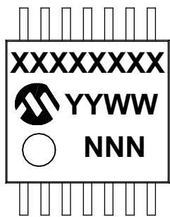
14-Lead TSSOP (4.4 mm) ( MCP6V79 )
