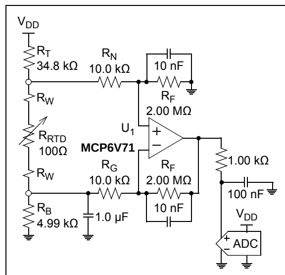
FIGURE 4-12: RTD Sensor.
