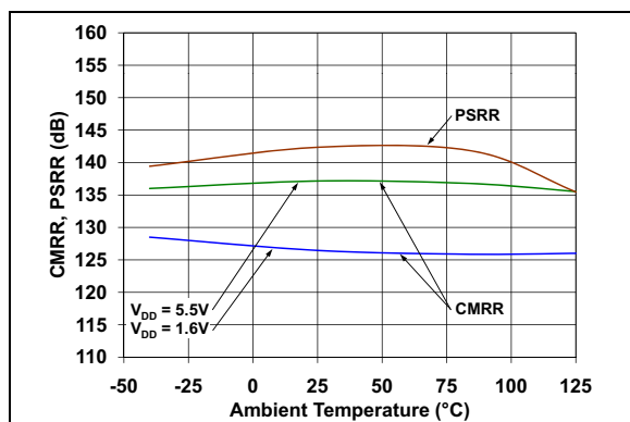
FIGURE 2-9: CMRR and PSRR vs. Ambient Temperature.
