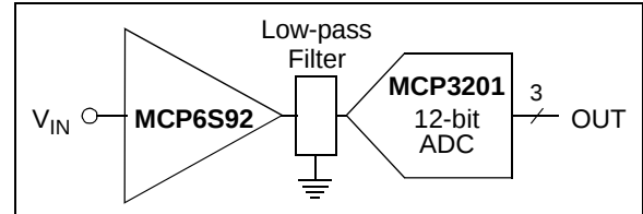
FIGURE 6-12: PGA as an ADC driver.
