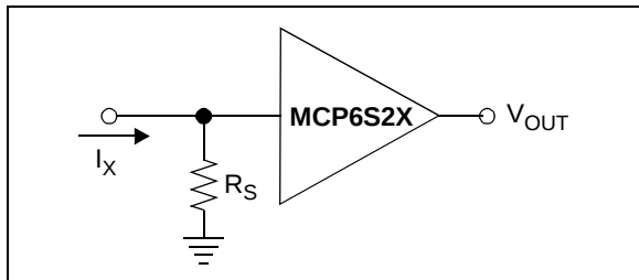
FIGURE 6-3: Wide Dynamic Range Current Measurement Circuit.
