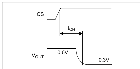
FIGURE 1-1: Channel Select Timing Diagram.
