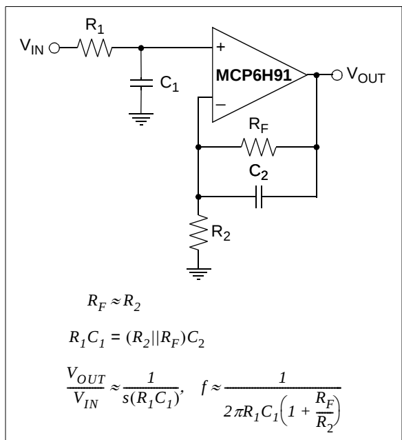
FIGURE 4-10: Non-Inverting Integrator.
