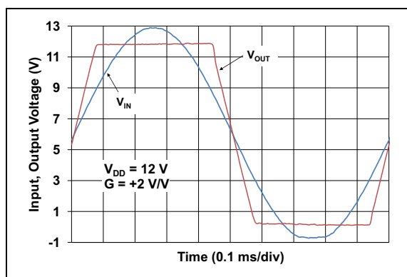
FIGURE 2-36: The MCP6H91/2/4 Shows No Phase Reversal.
