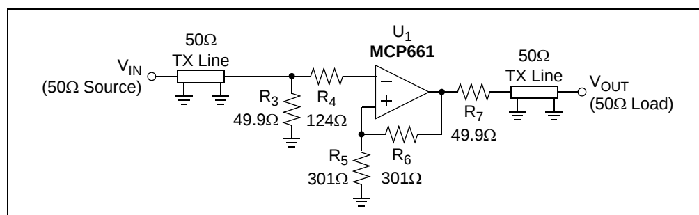
FIGURE 1-2: Simplified Circuit Diagram.
