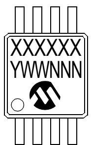
8-Lead MSOP (MCP6562)
