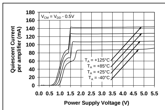
FIGURE 2-15: Quiescent Current vs. Power Supply Voltage.
