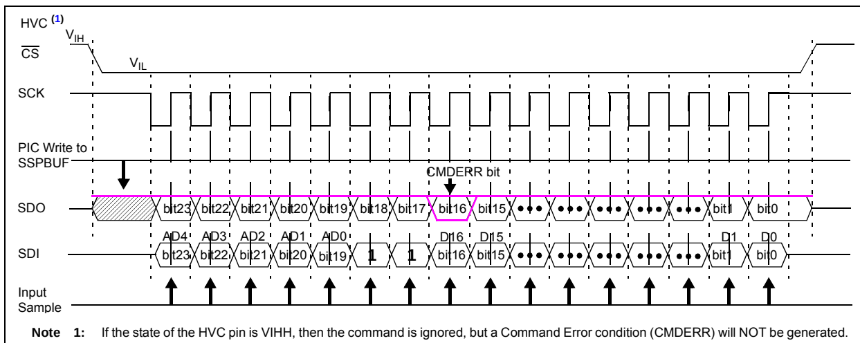
FIGURE 7-8: 24-Bit Read Command (C1:C0 = "11") - SPI Waveform with PIC MCU (Mode 1,1).
