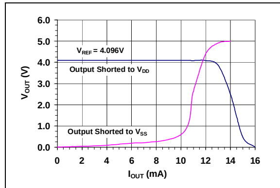
FIGURE 2-28: I_{OUT} vs. V_{OUT} . Gain = 2\times .
