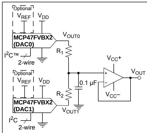
FIGURE 8-7: Simple Double Precision DAC using MCP47FVBX2.
