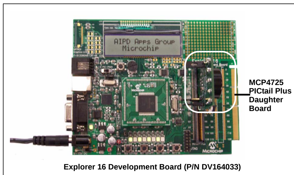
FIGURE 1-2: Connecting the MCP4725 PICtail™ Plus Daughter Board to the Explorer 16 Development Board.
