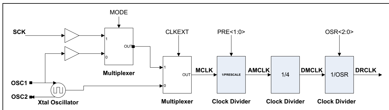
FIGURE 4-1: Clock Sub-Circuitry.
