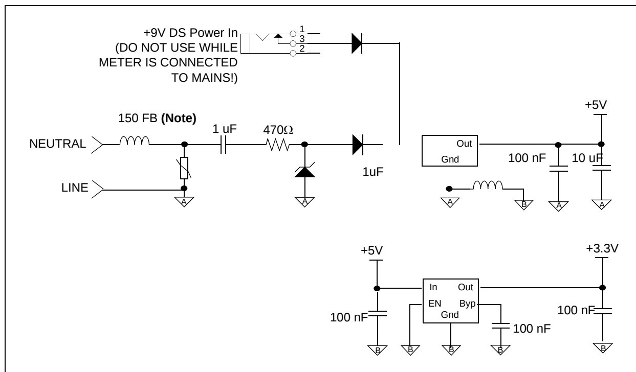
FIGURE 2-2: Low-Cost Power Supply Circuit.
