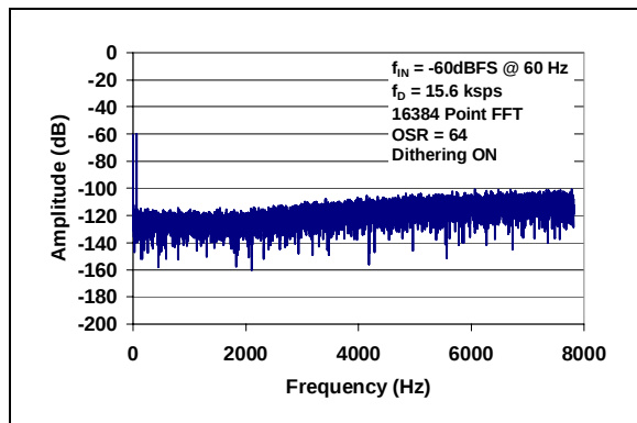
FIGURE 2-8: Spectral Response.
