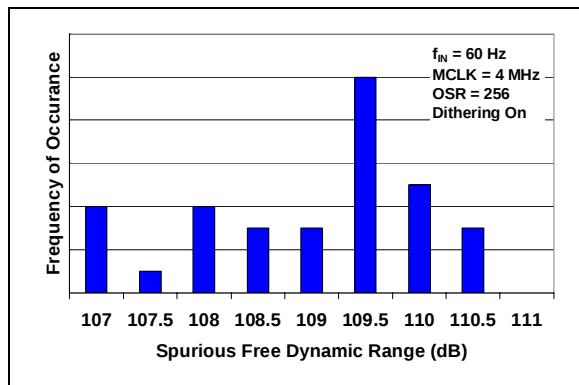
FIGURE 2-9: Spurious Free Dynamic Range Histogram.
