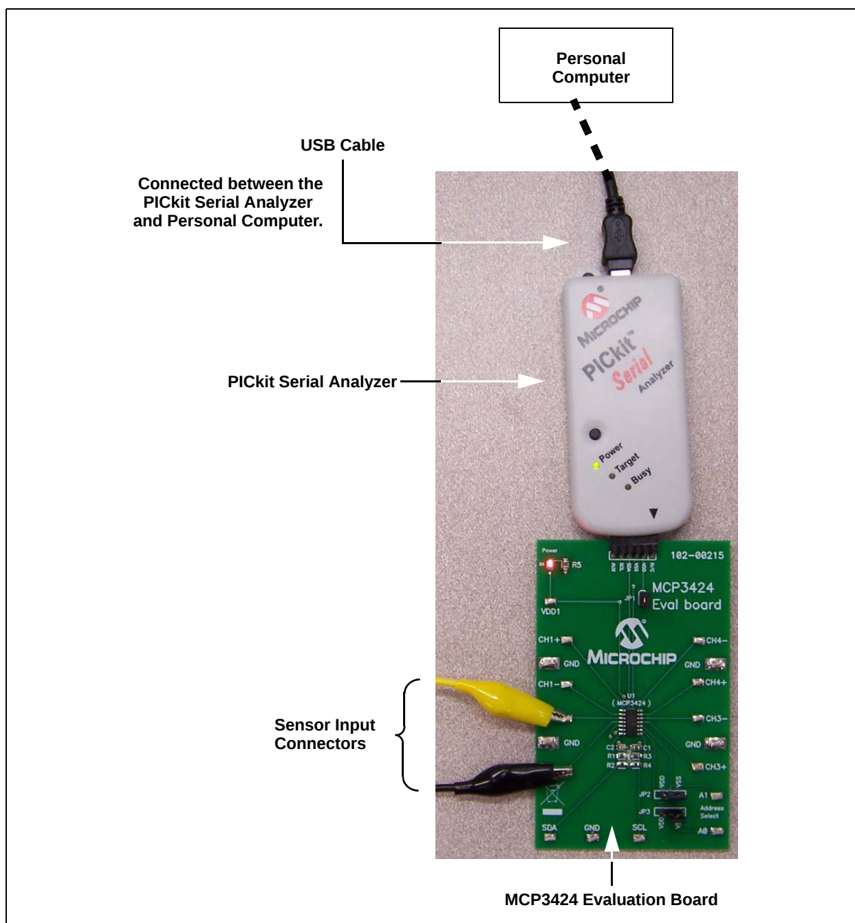
FIGURE 1-2: MCP3424 Evaluation Board with the PICkit Serial Analyzer.
