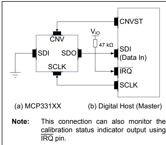
FIGURE 6-5: Connection Diagram for 3-Wire \overline{\text{CS}} Mode with \overline{\text{BUSY}} Status Indicator Output Bit. \overline{\text{IRQ}} Pin in the Host Device Is Used for Interrupt Event.
