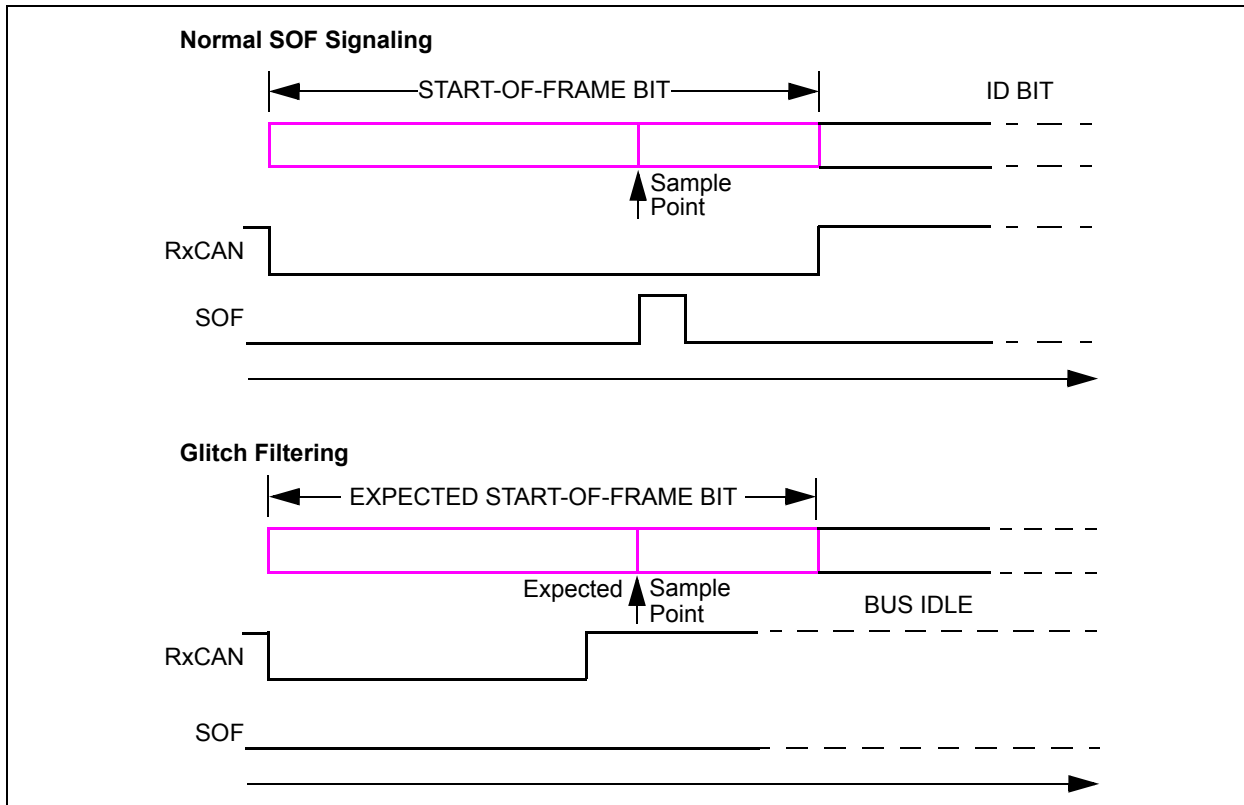
FIGURE 3-5: START-OF-FRAME SIGNALING
