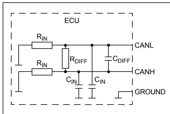
FIGURE 7-10: PHYSICAL LAYER DEFINITIONS
