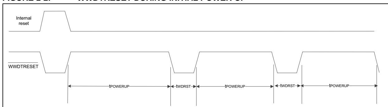
FIGURE 1-2: WWDTRESET DURING INITIAL POWER-UP
