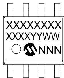
8-Lead SOIC (150 mil) ( MCP2021, MCP2021P )
