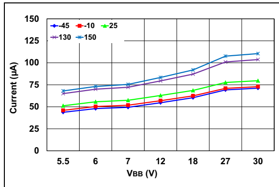
FIGURE 2-1: Typical I_{BBQ} .
