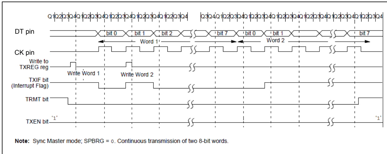
FIGURE 28-8: SYNCHRONOUS TRANSMISSION
