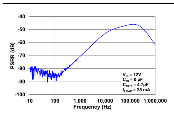
FIGURE 7-8: Internal LDO PSRR vs. Frequency.
