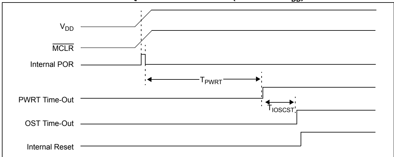
FIGURE 12-6: TIME-OUT SEQUENCE ON POWER-UP (MCLR WITH V DD )
