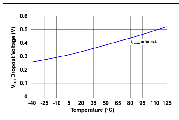
FIGURE 7-7: Internal LDO Dropout Voltage vs. Temperature.
