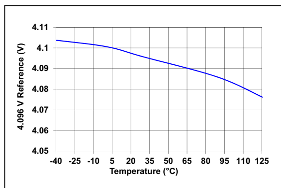
FIGURE 7-9: Internal ADC Reference Voltage vs. Temperature.
