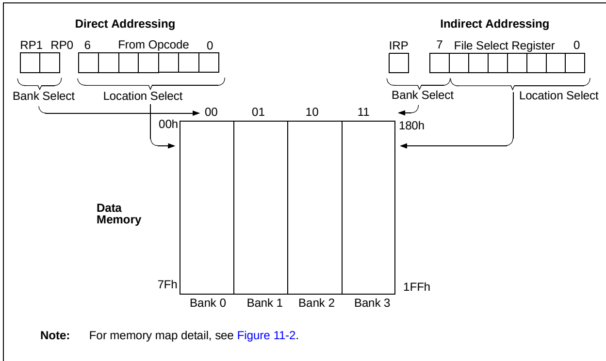
FIGURE 11-3: DIRECT/INDIRECT ADDRESSING
