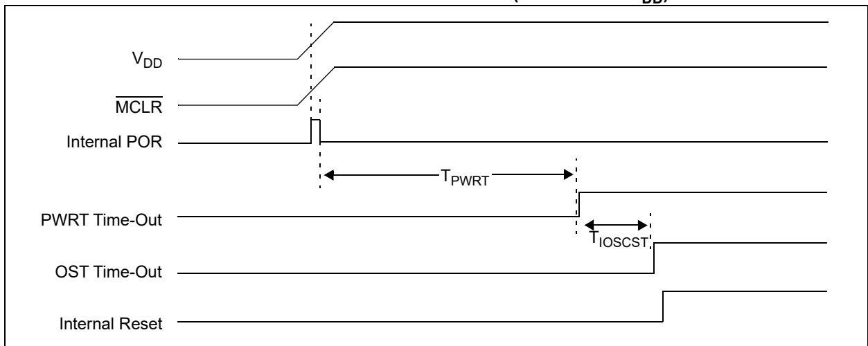
FIGURE 14-6: TIME-OUT SEQUENCE ON POWER-UP (MCLR WITH VDD)
