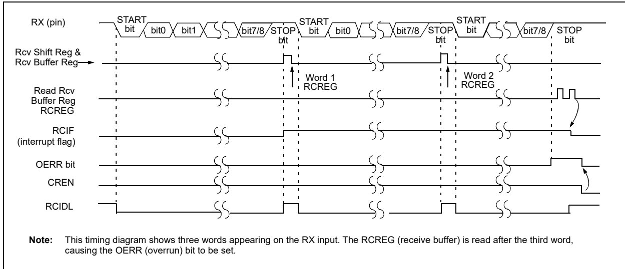
FIGURE 10-5: ASYNCHRONOUS RECEPTION
