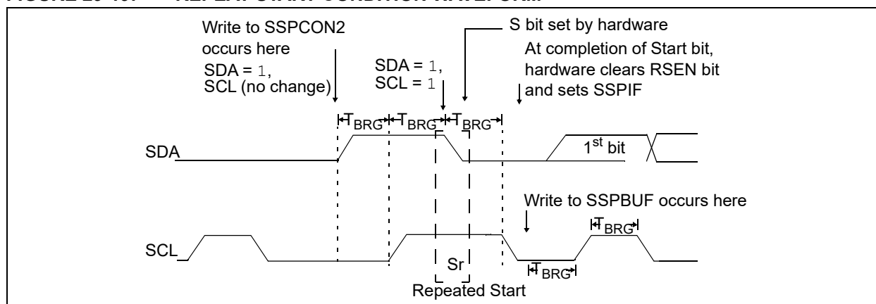
FIGURE 29-19: REPEAT START CONDITION WAVEFORM
