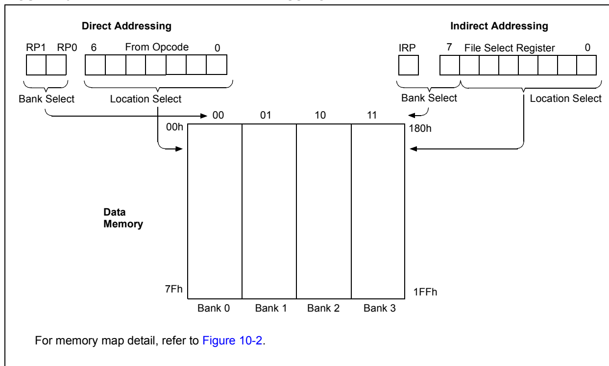
FIGURE 10-4: DIRECT/INDIRECT ADDRESSING
