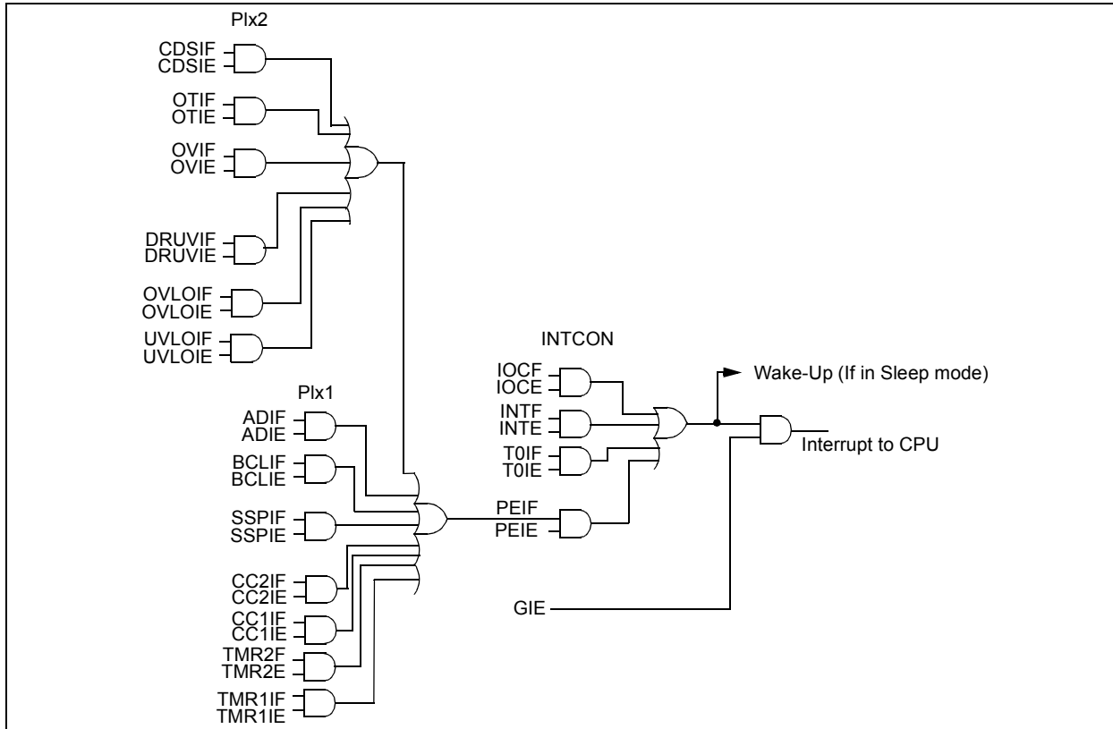
FIGURE 14-1: INTERRUPT LOGIC
