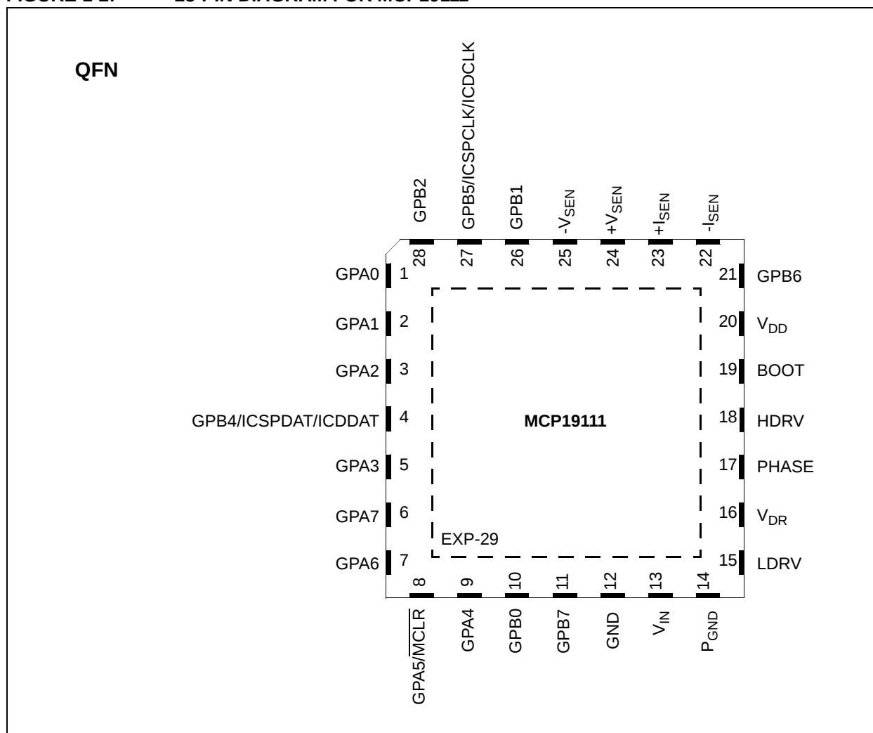
FIGURE 1-2: 28-PIN DIAGRAM FOR MCP19111
