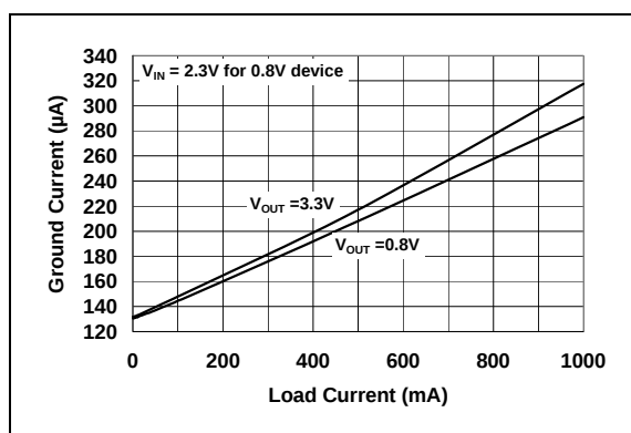
FIGURE 2-12: Ground Current vs. Load Current.
