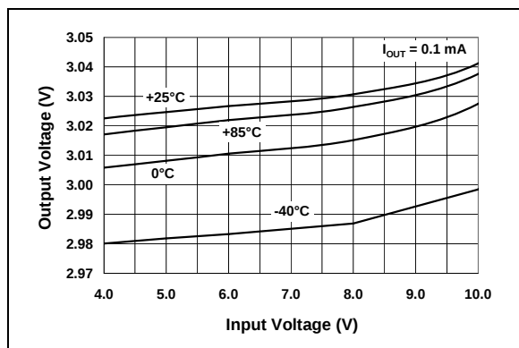
FIGURE 2-8: Output Voltage vs. Input Voltage ( V_R = 3.0V ).
