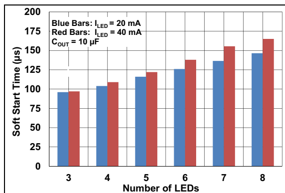
FIGURE 2-10: Start-Up Time vs. LED Number.
