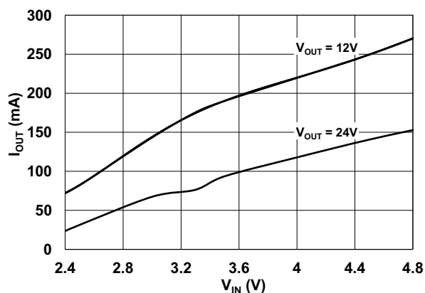
Maximum Output Current vs. V_{IN}
