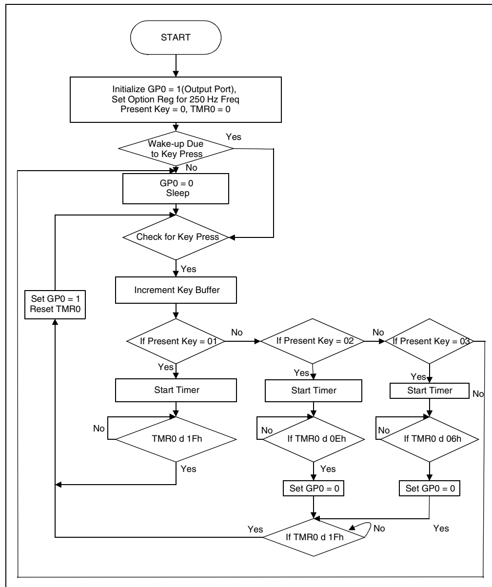
FIGURE C-1: Firmware Flowchart – Page 1.
