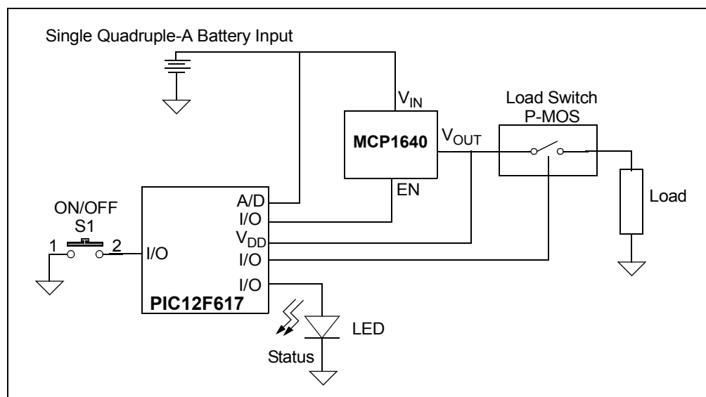
FIGURE 2-1: MCP1640 Single Quadruple-A Battery Boost Converter Reference Design Block Diagram.
