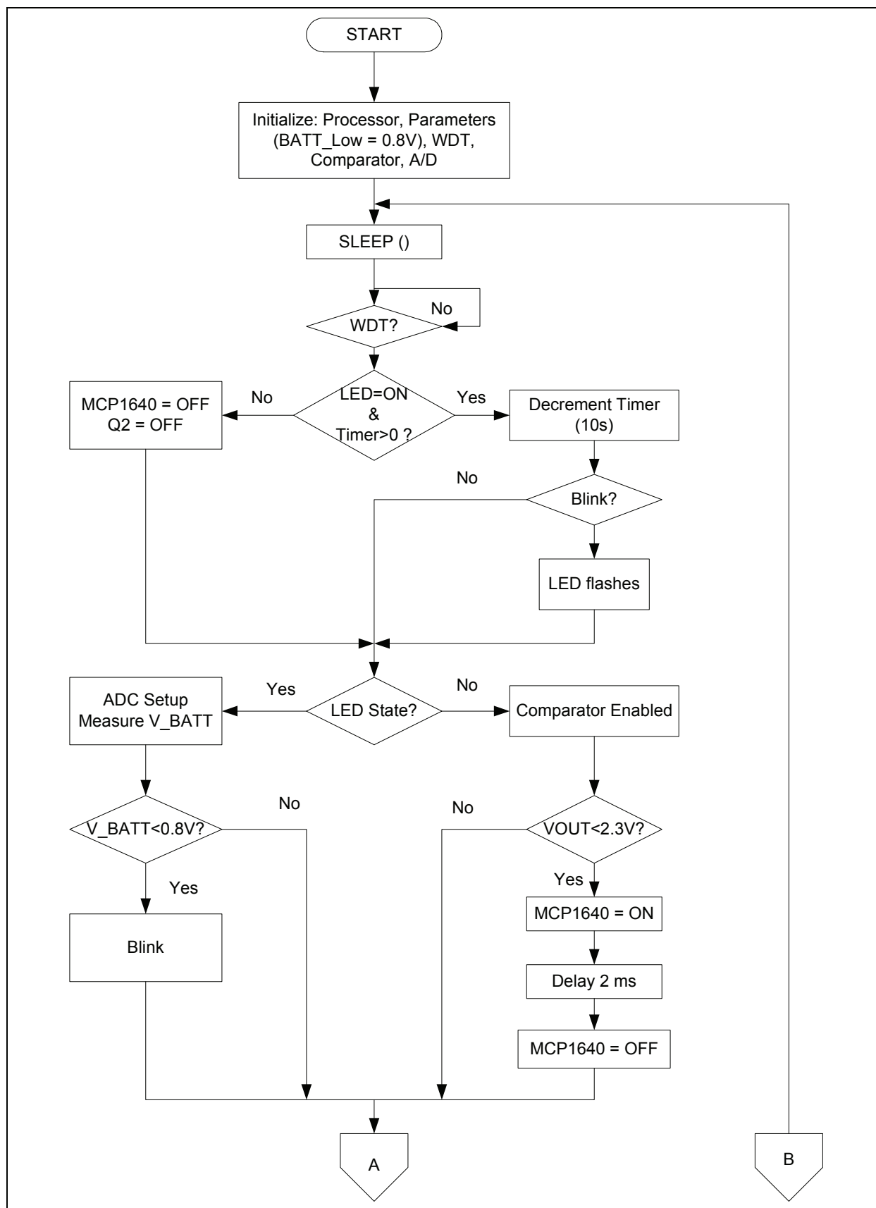
FIGURE C-1: Firmware Flowchart.
