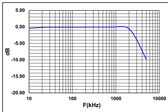
FIGURE 2-31: Error Amplifier BW at V_{DD}=5V .
