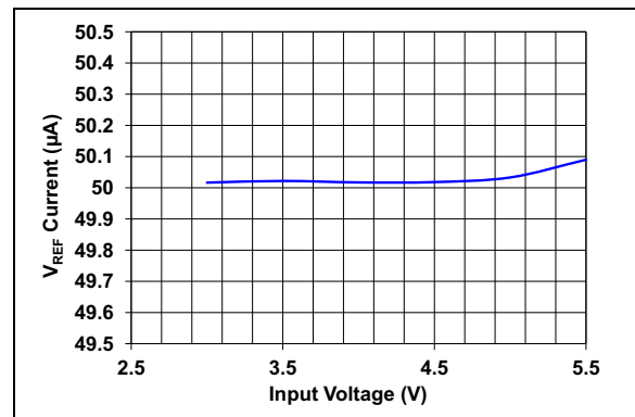
FIGURE 2-5: V_{REF} Current vs. Input Voltage.
