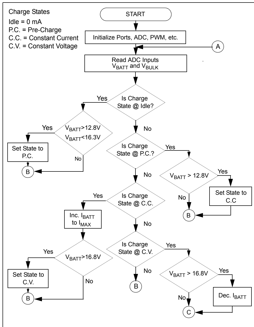
FIGURE C-1: Firmware Flowchart, page 1.
