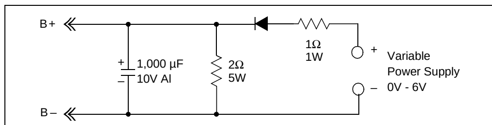
FIGURE 2-2: Simulated Battery Load.
