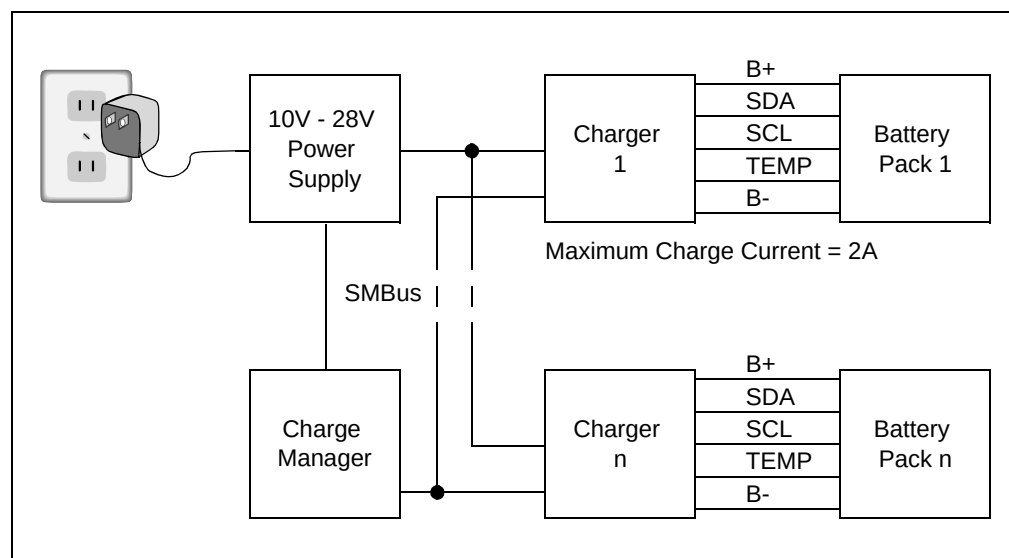
FIGURE 1-1: MCP1630 Li-Ion Multi-Bay Battery Charger Block Diagram.
