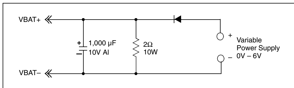
FIGURE 2-2: Simulated Battery Load.
