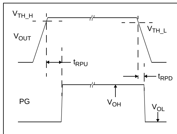
FIGURE 4-1: Power-Good Timing.
